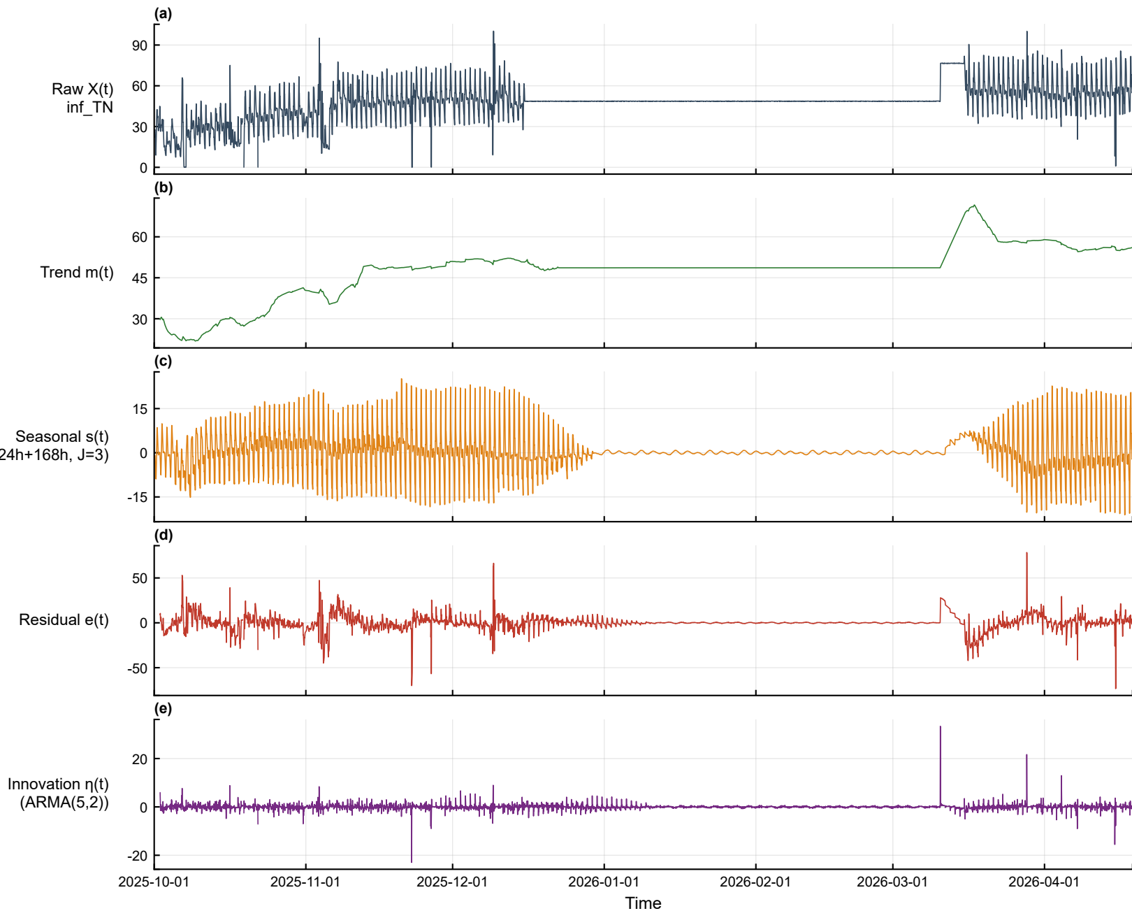
Multi-scale decomposition — inf_TN (influent, hour) [2025-10-01~2026-04-19]
